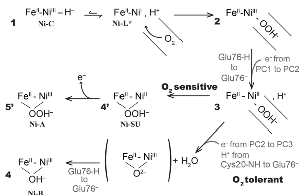
Scheme 1. Proposed reaction mechanism against O 2 -induced oxidative stress at the active site of hydrogenases. The 4' and 5' species are depicted with bridging peroxides, which could also be OH - /SO. [8b] The active site is represented by the bimetallic center, and events that occur at the proximal cluster are shown in gray.
